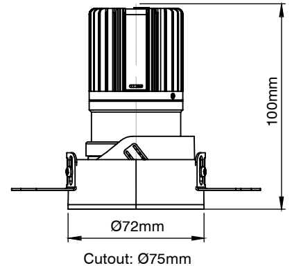
Cutout: Ø75mm
